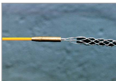
Flexible: the revolving threaded sleeve connects cable grip and rod.
